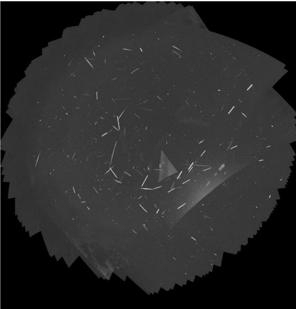
Sporadic meteors on 3 rd /4 th january
